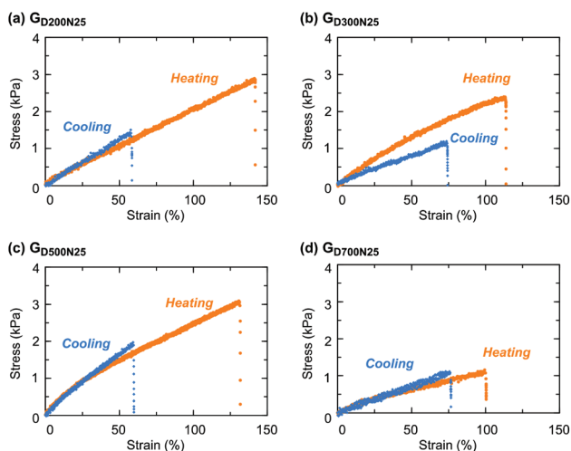
Fig. 4 Uniaxial tensile tests of the gels with a CD structure in heating and cooling states prepared from various macro-CTAs with different molecular weights: (a) G D200N25 , (b) G D300N25 , (c) G D500N25 , and (d) G D700N25 .
