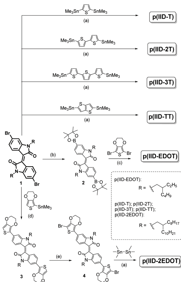
Scheme 2 Synthesis of isoindigo-polymers p(IID-T) , p(IID-2T) , p(IID-3T) , p(IID-TT) , p(IID-EDOT) and p(IID-2EDOT) . Reagents and conditions: (a) Pd(PPh 3 ) 4 , toluene, 100 \text{ }^\circ\text{C} for 24 h; (b) \text{B}_2(\text{Pin})_2 , KOAc, Pd(dppf) \text{Cl}_2 \cdot \text{DCM} , 1,4-dioxane, 80 \text{ }^\circ\text{C} for 18 h; (c) Pd(PPh 3 ) 4 , K 2 CO 3 in H 2 O, toluene, 85 \text{ }^\circ\text{C} for 72 h (d) Pd(PPh 3 ) 4 , toluene, 90 \text{ }^\circ\text{C} for 16 h; (e) NBS, THF, 0 \text{ }^\circ\text{C} to r.t. for 24 h.
