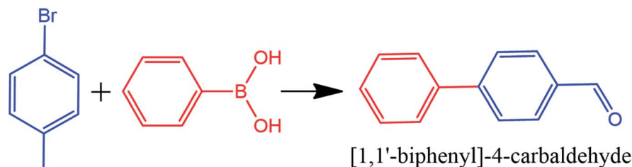
Fig. 4 Suzuki cross-coupling reaction with Pd-Fe 3 O 4 /RGO heterogeneous catalyst. This figure was adapted with permission from H. A. Elazab, 2019 (DOI: 10.9767/bcrec.14.3.3518.478-489). 50
