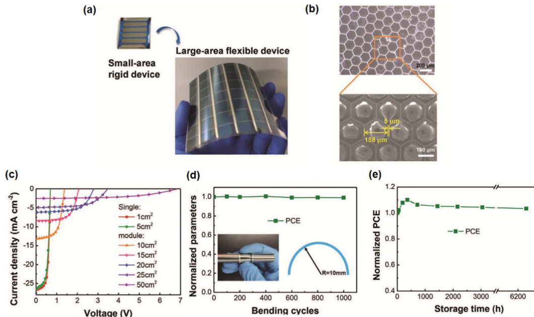
Fig. 17 (a) The small area rigid device and large-area flexible device. (b) Optical microscopy and SEM images of the PET/silver-grid substrate. (c) J - V curves of the PTB7-Th:Co 8 DFIC:PC 71 BM film coated by the slot-die method with different device areas. (d) Bending stability test. (e) Storage stability of devices in a nitrogen glove box. Adapted with permission. 152 Copyright 2020, Wiley-VCH Verlag GmbH & Co. KGaA.
