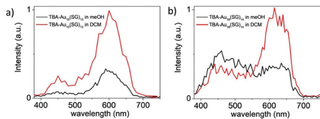
Fig. 15 Two-photon excited fluorescence spectra for (a) \text{TBA-Au}_{15}(\text{SG})_{13} and (b) \text{TBA-Au}_{18}(\text{SG})_{14} at the excitation wavelength of 780 nm. Reproduced with permission. 180 Copyright 2018. Wiley-VCH.
