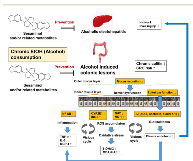
Fig. 10 Hypothesis of the preventive effects of sesaminol and/or related metabolites against ethanol-oxidative stress in the colon.
