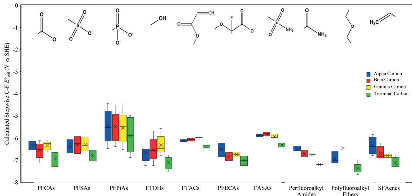
Fig. 4 Theoretically calculated E_{red,eq}^0 values for the cleavage of a C-F bond at different positions of various PFASs. The E_{red,eq}^0 values were calculated based on M06-2X/cc-pVDZ.
