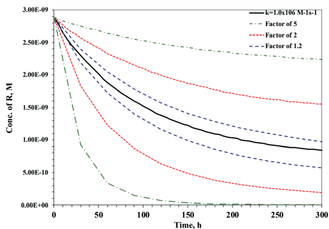
Fig. 5 Time-dependent concentration of a target compound with k_{chem} = 1.0 \times 10^6 \text{ M}^{-1} \text{ s}^{-1} and different predicted values by a difference of a factor of 1.2, 2, and 5 in UV/sulfite process. 10
