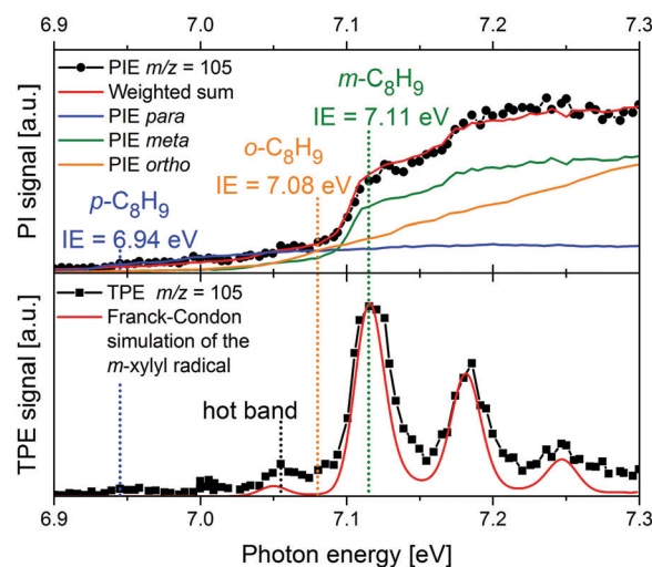
Fig. 8 In a m -xylene flame, m/z 105 was identified, corresponding to xyllyl radicals. The photoion signal (upper trace) does not permit identification of the product isomer. The TPE spectrum in the lower trace, on the other hand shows that meta -xyllyl is the dominant product isomer and the band around 7.05 eV assigned to a hot band. The Figure was published in ref. 151, Copyright Elsevier, 2017.
