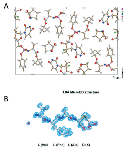
Fig. 8 (A) The structural model of sofosbuvir L-proline cocrystal determined by PEDT. Reproduced from ref. 111 with permission from the American Association for the Advancement of Science, copyright 2019. (B) MicroED structure of the D configuration of the 3-thiaGlu in the chemically synthesized tetrapeptides (VFAX, X = 3-thiaGlu). Reproduced from ref. 112 with permission from the American Association for the Advancement of Science, copyright 2019.
