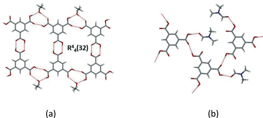
Fig. 7 (a) H_3btc \cdot EtOH solvate which shows typical layer formed in alcohol solvates with [ChemTemp] 46 ; (b) disruption of the layer in the 2:1 H_3btc \cdot DMF solvate (XAVPOZ 47 ) (adapted from ref. 44).
