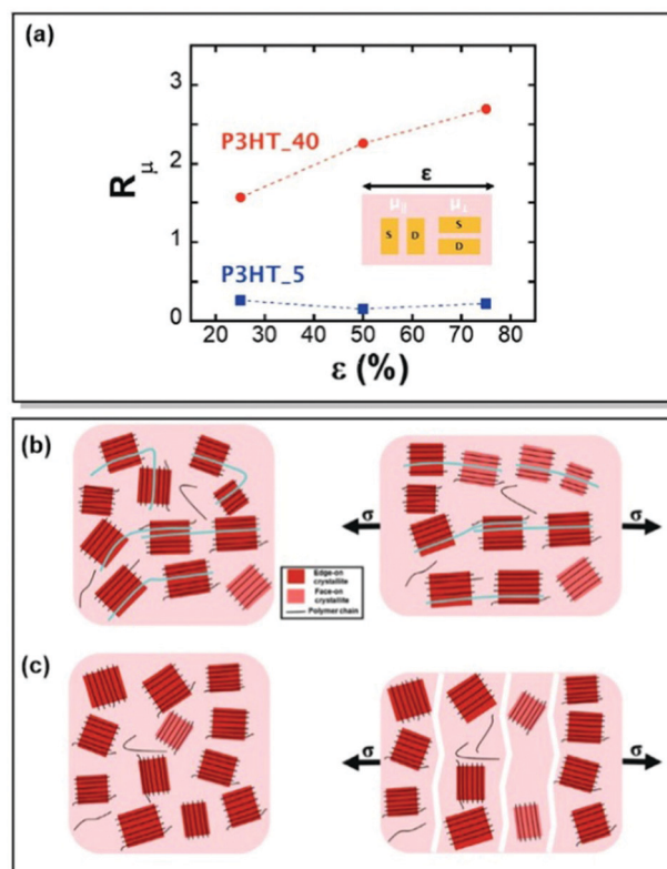
Fig. 11 (a) Anisotropy in the field-effect mobility ( R_{H,i} ) of transistors utilizing P3HT_40 and P3HT_5 thin films, as a function of strain. Schemes of unstrained and strained (b) P3HT_40 and (c) P3HT_5 , highlighting the role of tie chains between the crystallites on polymer morphology upon strain. Reproduced with permission from Wiley. 91
