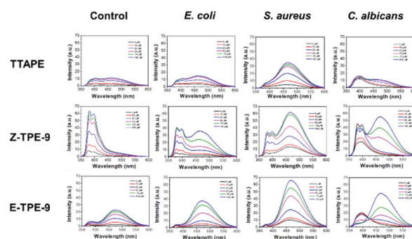
Fig. 1 Fluorescence spectra of TTAPE, Z-TPE-9 and E-TPE-9 (5, 10, 25, 50, 75, and 100 \mu\text{M} ) with the addition of \text{Amp}^r E. coli , S. aureus and C. albicans after 30 min of incubation, respectively.
