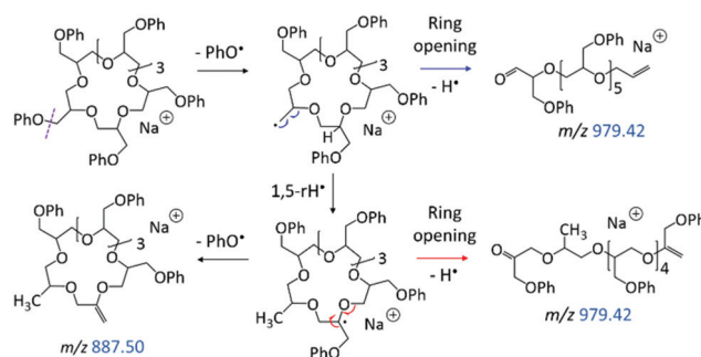
Scheme 2 Homolytic ring-opening of sodiated \text{C}_7 ( m/z 1073.47), initiated by \text{PhO}^\bullet loss. Smaller fragment ions are attributed to the ring-opened structures (Schemes 3–4).
