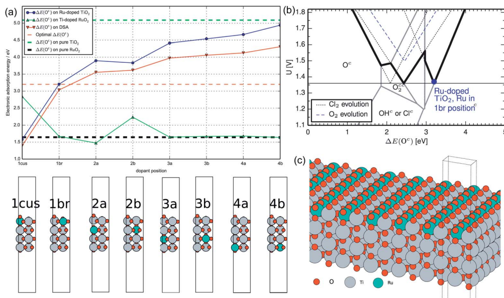
Fig. 5 (a) Covered oxygen adsorption energy \Delta E(\text{O}_2) for Ru-doped \text{TiO}_2 , Ti-doped \text{RuO}_2 , DSA and pure \text{RuO}_2 and \text{TiO}_2 at different dopant positions from DFT modelling. (b) Volcano plot from Hansen's work in collaboration with Ru-doped \text{TiO}_2 at the '1br' site (bold line) in this work. (c) A unit model of the optimized identical Ru-doped \text{TiO}_2 surface. Reproduced with permission. 56 Copyright 2014, Elsevier.
