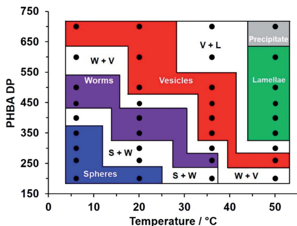
Fig. 7 Variable temperature phase diagram constructed for a series of linear \text{PEG}_{113} - \text{PHBA}_x nano-objects prepared via RAFT aqueous dispersion polymerization of HBA targeting 15% w/w solids. Copolymer morphologies were initially assigned on the basis of visual appearance and corroborated by SAXS (Fig. 4c and S8†), TEM (Fig. 3, 4b and 5d) and rheological studies (Fig. 5 and S11†). [N. B. S + W, W + V and V + L denote mixed phases comprising spheres plus worms, worms plus vesicles or vesicles plus lamellae, respectively].
