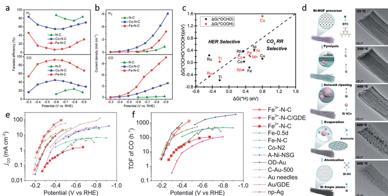
Fig. 2 The Faradaic efficiencies for \text{CO} and \text{H}_2 (a) and the current densities (b) of N–C, Co–N–C, and Fe–N–C. Reproduced from ref. 58 with permission from the American Chemical Society, copyright 2018. (c) Gibbs free energy changes for the first protonation step. Reproduced from ref. 63 with permission from The Royal Society of Chemistry, copyright 2018. (d) A schematic illustration of the process of Bi-MOF transformation to single Bi atoms and TEM images of Bi-MOF pyrolyzed at different temperatures. Reproduced from ref. 64 with permission from the American Chemical Society, copyright 2019. (e) \text{CO} current density ( j_{\text{CO}} ) and (f) apparent TOFs of \text{CO} production of \text{Fe}^{3+} -N–C and of \text{Fe}^{2+} -N–C in comparison with other reported catalysts. Reproduced from ref. 59 with permission from the American Association for the Advancement of Science, copyright 2019.
