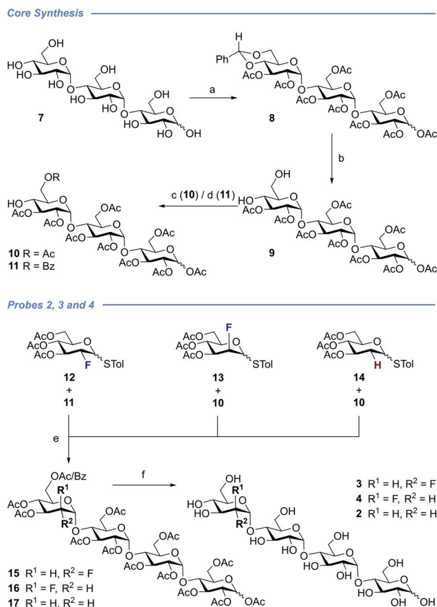
Scheme 1 Preparation of fluorinated maltotetraose cores 3 and 4 , and the control system 2 . Conditions: (a) (1) Benzaldehyde dimethyl acetal, p -TsOH, DMF, 4 h, 50 °C, 150 mbar; (2) Ac 2 O, DMAP, pyridine, 4 h, RT, 69% over two steps. (b) TFA/H 2 O (10 : 1), CH 2 Cl 2 , RT, 98%. (c) Acetyl chloride, HOBt, TEA, CH 2 Cl 2 , RT, 76%. (d) Benzoyl chloride, pyridine, 3 h, -10 °C, 57%. (e) NIS, TMSOTf, CH 2 Cl 2 , 15 min, RT, 15 : 33%, 16 : 50%, 17 : 11%. (f) NaOMe, MeOH, RT, 3 : 69%, 4 : 86%, 2 : 94%.
