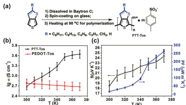
Fig. 12 (a) Synthesis and structural formula of PTT-Tos; (b) temperature-dependent conductivity of PTT-Tos compared with PEDOT-Tos; (c) temperature-dependent Seebeck coefficient and power factor of PTT-Tos. Reproduced from ref. 99 with permission from John Wiley and Sons.
