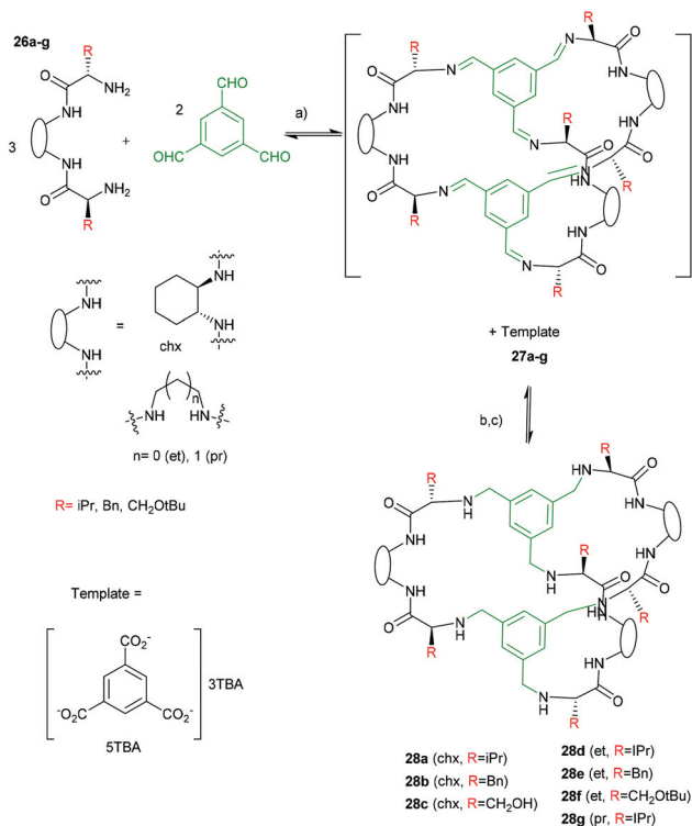
Scheme 1 Synthesis of pseudopeptidic cages described by Alfonso. 98 (a) Equilibrium at RT either in the absence or the presence of 5TBA. (b) BH 3 .py (c) HCl.
