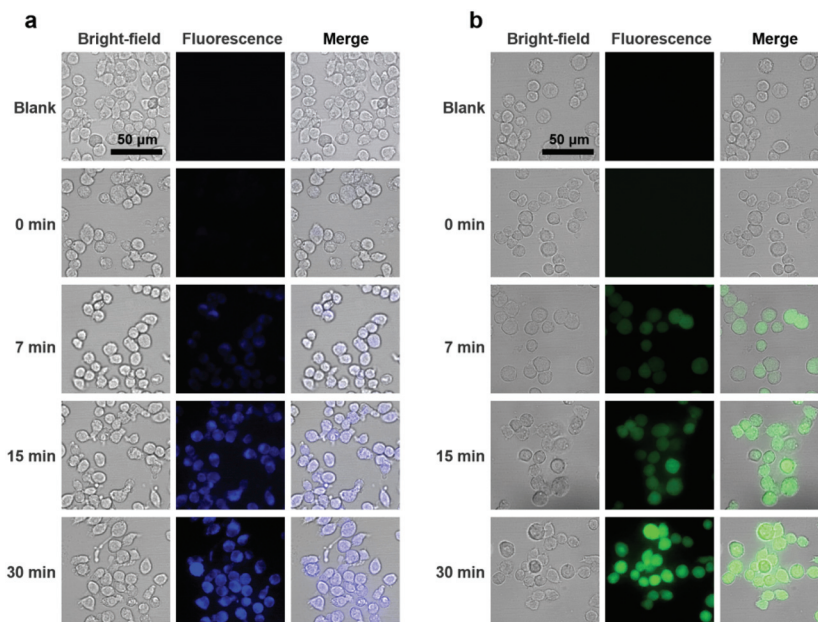
Fig. 5 Detection of \text{H}_2\text{S} by DS-Blue-Nano and DN-Green-Nano in living macrophage cells. Cells were treated with \text{Na}_2\text{S} ( 100 \mu\text{M} ) to generate exogenous \text{H}_2\text{S} , untreated cells were used as control. The cells were then incubated with DS-Blue-Nano ( 10 \mu\text{M} , as a) or DN-Green-Nano ( 10 \mu\text{M} , as b). The photos were taken under a fluorescent microscope. Scale bar: 50 \mu\text{m} .
