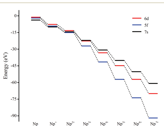
Scheme 1 Smearred energies of the valence atomic orbitals of \text{Np}^{n+} ( n = 0 to 7).
