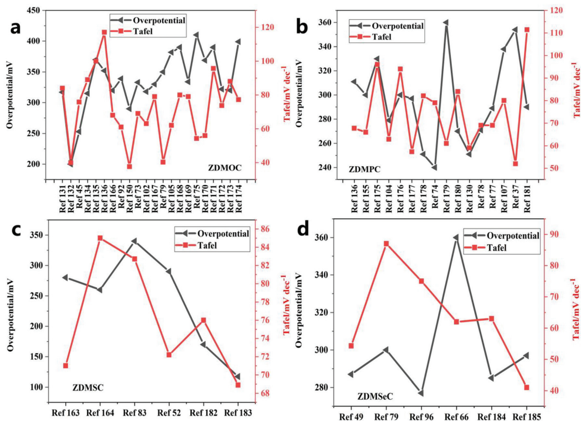
Fig. 22 Comparison of the Tafel slopes and the overpotentials of different catalysts of (a) ZDMOC, (b) ZDMPC, (c) ZDMS and (d) ZDMSeC at a current density of 10 \text{ mA cm}^{-2} .
