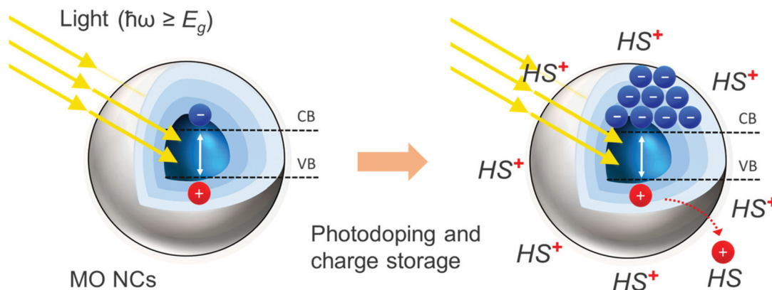
Fig. 1 Photodoping and multiple charge accumulation in doped MO NCs. Light absorption with energy ( \hbar\omega ) above the bandgap ( E_g ) promotes an electron from the valence band (VB) to the conduction band (CB). By removing the photo-generated hole with a hole-scavenger (HS), the electron-hole pair recombination is suppressed and the extra electron is stored in the nanocrystal. The absorption of several photons results in the accumulation of multiple photoelectrons in the NC and leads to the overall photodoping of the material.
