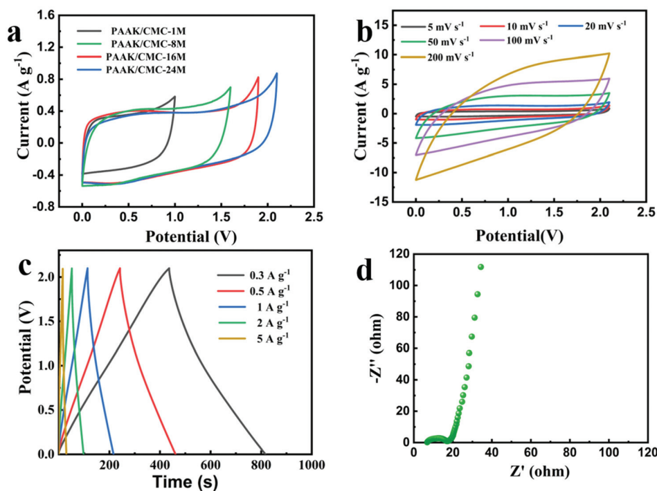
Fig. 3 Voltage windows of PAAK/CMC-1, 8, 16, 24 M at 5 mV s -1 (a), CV curves from 5 mV s -1 to 200 mV s -1 (b), GCD profiles from 0.3 A g -1 to 5 A g -1 (c) and EIS (d) of the NG//NG quasi-solid-state supercapacitor with the PAAK/CMC-24 M polyelectrolyte hydrogel.
