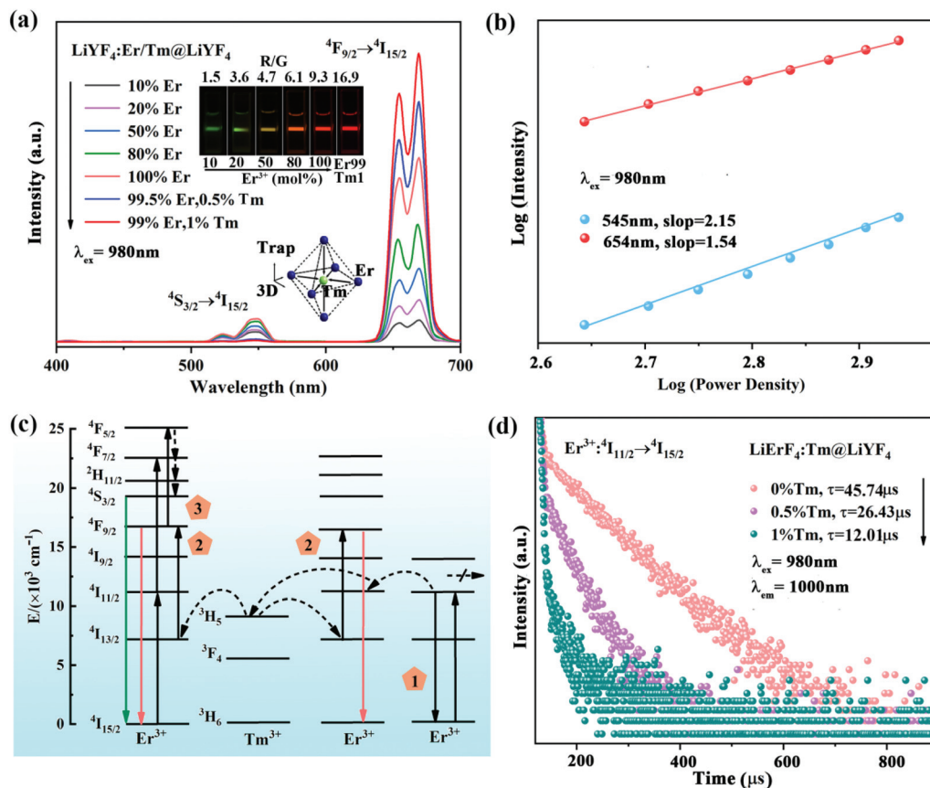
Fig. 2 (a) Upconversion spectra of the as-obtained LiYF 4 :Er 3+ /Tm 3+ @LiYF 4 nanoparticles doped with different concentrations of Er 3+ and Tm 3+ . Inset: the photographs of the colloidal dispersion of the corresponding samples under excitation with a 980 nm laser diode, and a structural model for Tm 3+ -mediated energy condensation between Er 3+ ions. (b) Power density dependence of the 545 and 654 nm emission, indicating a two-photon population process for the red emission and a three-photon population process for the green emission in the LiErF 4 :1%Tm 3+ @LiYF 4 nanocrystals under 980 nm excitation. (c) Proposed upconversion mechanism for LiErF 4 :1%Tm 3+ @LiYF 4 nanoparticles. (d) The luminescence decay curves of Er 3+ of LiYF 4 :Tm 3+ @LiYF 4 with different Tm 3+ concentrations.
