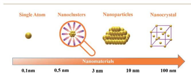
Fig. 1 Size scale from single atoms to nanocrystals.
