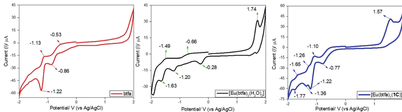
Fig. 7 Cyclic voltammograms of btfa (red), [Eu(btfa) 3 (H 2 O) 2 ] (black) and [Eu(btfa) 3 ] 1c (blue) in the region between -2.0 to 2.0 V on glassy carbon electrode in 0.1 M Bu 4 NPF 6 solution in DCM at a scan rate of 100 mV s -1 .
