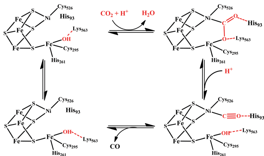
Scheme 4 Proposed mechanistic cycle of \text{CO}_2 reduction to CO by [\text{NiFe}] CODHs.
