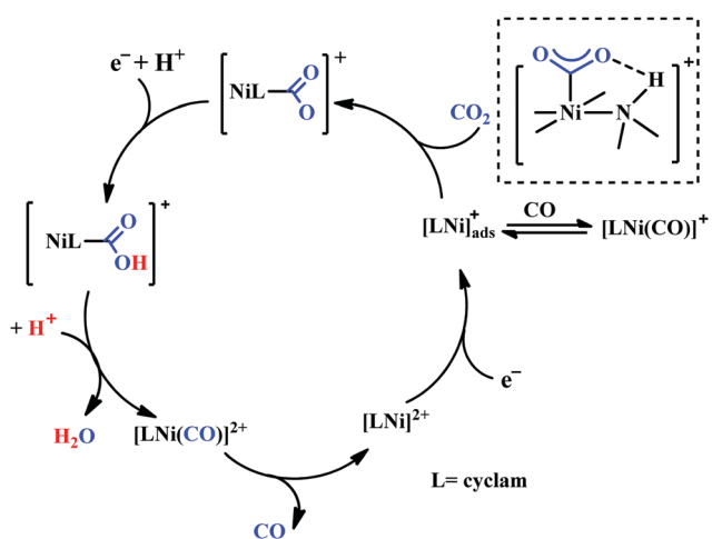
Scheme 12 Proposed mechanistic pathway of electrocatalytic CO 2 reduction to CO by [Ni II (cyclam)]-based macrocycles.
