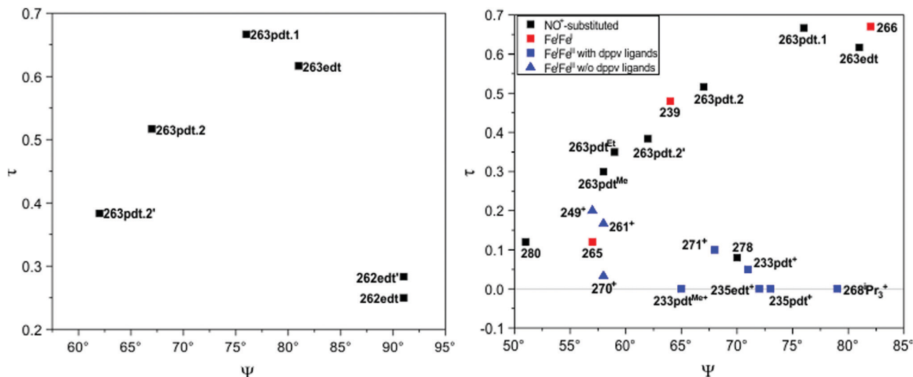
Fig. 78 Left: Addison's \tau parameter against \Psi for the nitrosyl complexes 262edt , 263edt and 263pdt . 263pdt.1 refers to the ba/ap rotamer and 263pdt.2 to the ba/ba rotamer. The ' denotes different independent molecules in the asymmetric unit. Both 263pdt.2 molecules are weakly disordered, but the angles vary only by 1°. For all molecules of 263pdt \tau was calculated with the semi-bridging carbonyl in apical position. Right: Addison's \tau parameter against \Psi for different rotated complexes.
