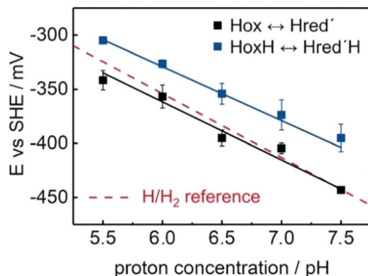
Fig. 14 Pourbaix diagram showing the transition potentials for H_{ox} \rightarrow H_{red}' (black) and H_{oxH} \rightarrow H_{red}'H (blue) as function of pH value. The slopes are 55 \pm 5 \text{ mV pH}^{-1} (black) and 50 \pm 3 \text{ mV pH}^{-1} (blue) with an approximate off-set of 50 mV that elevates the H_{oxH} \rightarrow H_{red}'H potential above the H/H 2 reference (red traces, 59 \text{ mV pH}^{-1} ). Error bars illustrate the quality of the Nernstian fit. Figure and caption are adopted with permission from reference. Reprinted from ref. 52 with permission from John Wiley and Sons, Copyright 2017.
