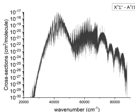
Fig. 12 Calculated absorption spectra of the \text{A } ^1\Pi - \text{X } ^1\Sigma^+ system at 2000\text{ K} with a Gaussian profile of HWHM = 1\text{ cm}^{-1} .
