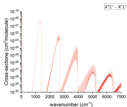
Fig. 11 Overview of the calculated \text{X } ^1\Sigma^+ state rotation-vibration absorption spectrum of PN at T = 2000\text{ K} with a Gaussian line profile of HWHM = 1\text{ cm}^{-1} .
