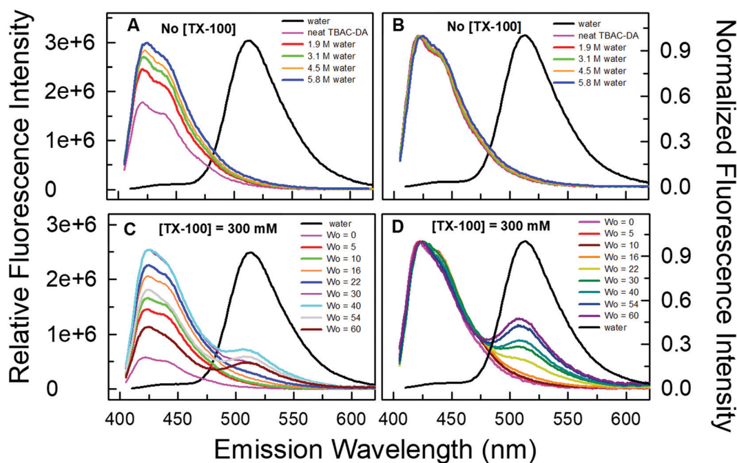
Fig. 4 Relative (panels A and C) and normalized (panels B and D) fluorescence emission spectra of pyranine (10 \mu\text{M} , \lambda_{ex} = 390 \text{ nm} , and slits: excitation/emission = 2/2 nm) dissolved within neat DES TBAC-DA and TX-100(300 mM)/TBAC-DA systems at different amounts of water loading ( w_0 ), respectively. The fluorescence emission spectrum of pyranine in water is also included in each panel for reference.
