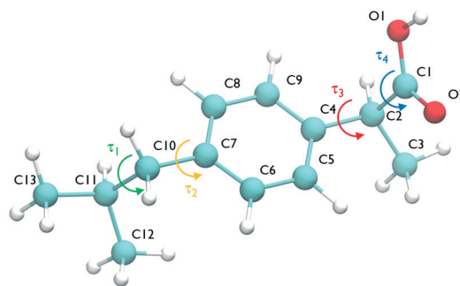
Fig. 1 The ibuprofen molecule showing atom labels and the four torsional angles considered in the crystal structure generation, namely \tau_1 (C12–C11–C10–C7), \tau_2 (C11–C10–C7–C8), \tau_3 (C5–C4–C2–C1) and \tau_4 (O1–C1–C2–C4).
