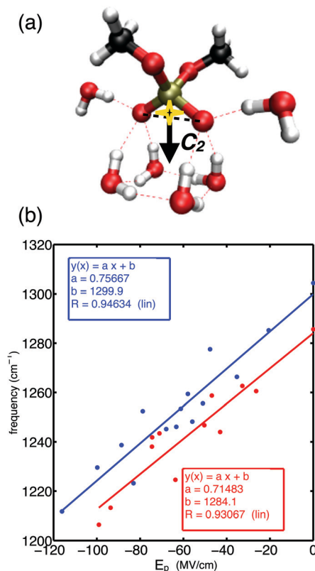
Fig. 1 (a) Molecular structure of dimethyl phosphate (DMP, (CH_3)_2PO_4^- ) together with an idealized first hydration shell of water molecules. The total electric field imposed by water molecules is projected on the bisector midpoint of the (PO_2)^- group in the direction of the angle bisector axis C_2 . (b) Correlation of the projected electric field E_p and the transition frequency of the asymmetric phosphate stretching vibration \nu_{AS}(PO_2)^- for DMP. \cdot xH 2 O molecular clusters ( x = 1-22 ), additionally shown are linear regressions of data points. Transition frequencies \nu_{AS}(PO_2)^- were evaluated in the harmonic approximation at density functional level of theory (PBE0 functional, blue) and many body perturbation theory (MP2, red). Adapted from ref. 60, with the permission of AIP Publishing.
