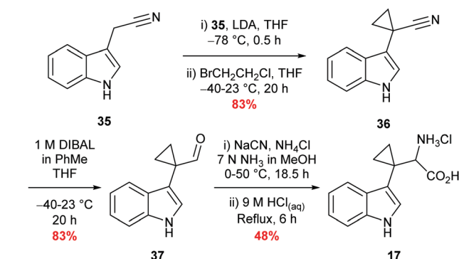
Scheme 5 Synthesis of \beta,\beta' -cyclopropyl tryptophan-mimic 17 .
