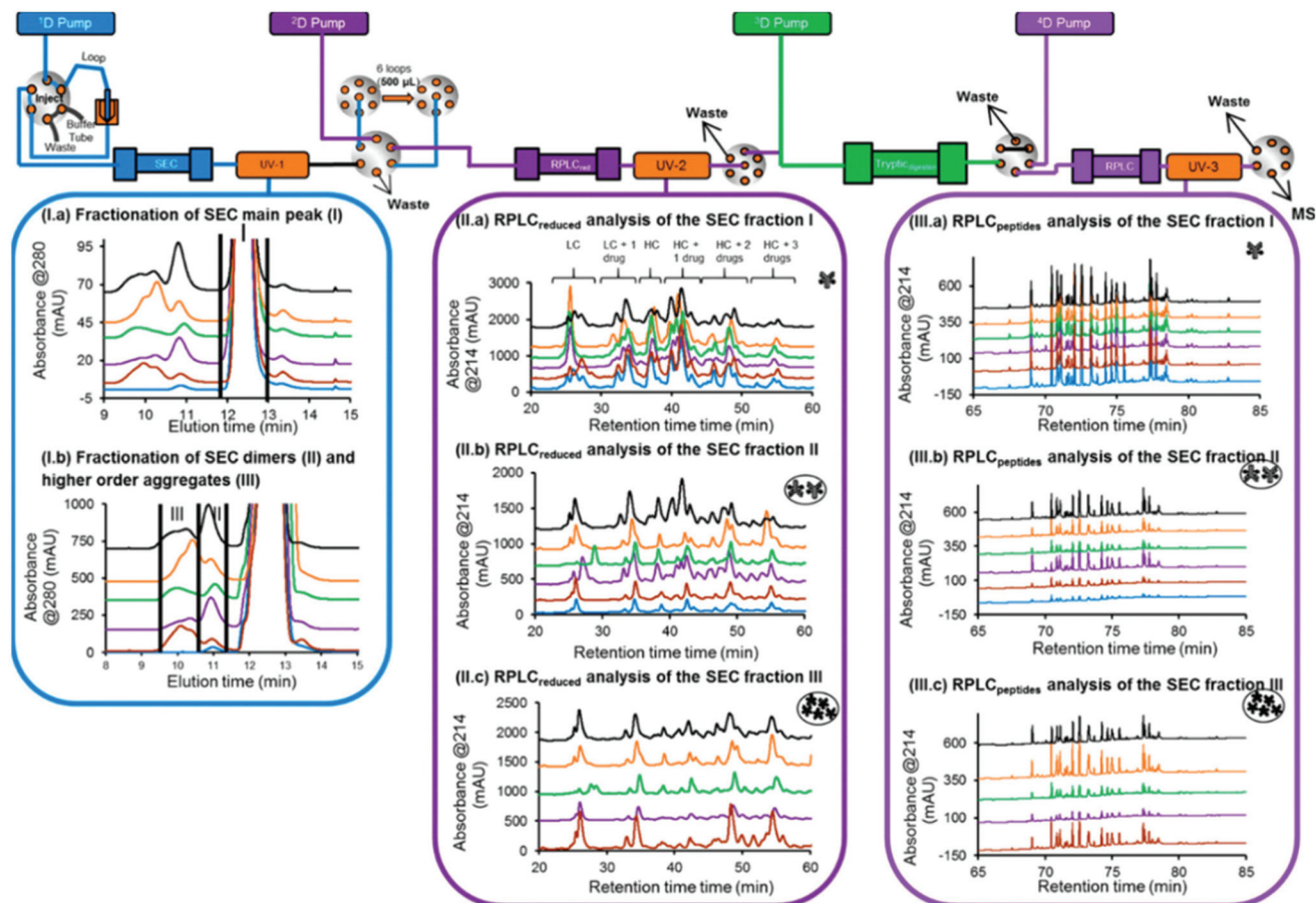
Fig. 5 Schematic representation of an automated 4D-LC-MS workflow for SEC coupled to online peptide mapping, enabling the separation and fractionation of size variants by SEC ( ^4D ) followed by on-column reduction by RPLC ( ^2D ), trypsin digestion in flow-through mode ( ^3D ), and peptide mapping analysis by RPLC ( ^4D ). (I, a, b) SEC of ADC product reference, and samples stressed thermally, by light, at basic pH, at acidic pH, and under oxidative conditions (blue, brown, purple, green, orange, gray, and black traces, respectively). (II, a–c) ^2D RPLC of the SEC heart-cut fractions that have been reduced online and then eluted. (III, a–c) ^4D RPLC of the SEC heart-cut fractions that have been reduced and trypsin digested online. Reproduced from A. Goyon, M. Kim, L. Dai, C. Cornell, F. Jacobson, D. Guillaume, et al., Streamlined Characterization of an Antibody–Drug Conjugate by Two-Dimensional and Four-Dimensional Liquid Chromatography/Mass Spectrometry, Anal. Chem. , 2019, 91, 2314896–14903. With permission from American Chemical Society, copyright 2019.
