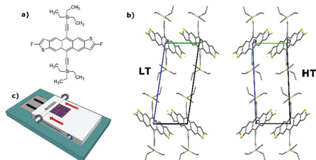
Fig. 1 (a) Molecular structure of diF-TES-ADT; (b) comparison of the two unit cells of the HT and LT polymorphs of diF-TES-ADT; (c) schematic representation of the BAMS apparatus.
