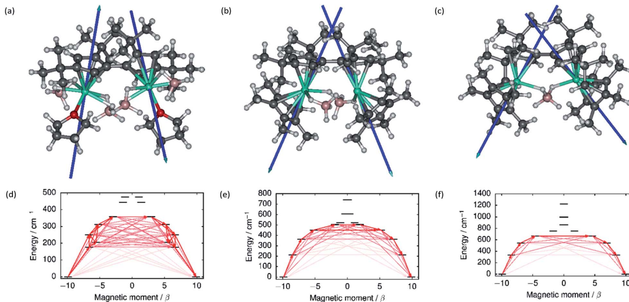
Fig. 3 The principal magnetic axes of the ground KDs of the Dy 3+ ions in (a) 1, (b) 2 and (c) 3. Calculated effective ab initio barriers for the relaxation of magnetization at the Dy1 ions (d) 1, (e) 2 and (f) 3. Stronger arrows indicate larger absolute value of the transition magnetic moment matrix elements between the respective states. Transitions involving higher-energy states not involved in the relaxation are omitted for clarity. The barriers for the Dy2 ions, which are similar to those of the Dy1 ions, are shown in ESI Fig. S25–S27.†
