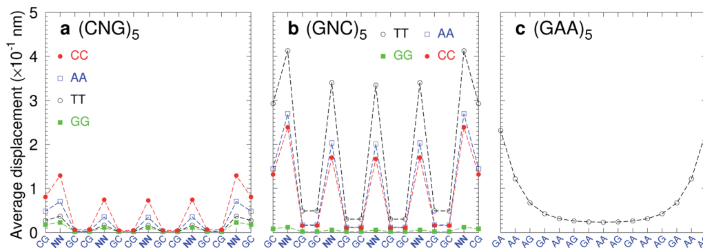
Fig. 13 Average displacements of tandem trinucleotide repeats of type (a) (CNG)_5 and (b) (GNC)_5 , with central mismatches AA (blue boxes), CC (red bullets), GG (green boxes) and TT (black circles). Panel (c) shows repeats of type (GAA)_5 formed solely of mismatches calculated with CI parameters. The calculation was carried out at 150 K, which has no relation to the melting temperatures.
