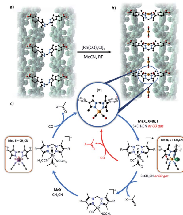
Fig. 7 Metalation of MnMOF-1 (a) with [Rh(CO) 2 Cl 2 ] yields MnMOF-1 [Rh(CO) 2 ][Rh(CO) 2 Cl 2 ] (b). The proposed catalytic cycle for the carbonylation of methyl iodide using the Rh(I) functionalised MOF is depicted (c) for both the gas phase (red) and solution phase (blue). R = MOF framework (MOF backbone – green surface, C – black, N – lavender, O – red, Rh – orange, I – green).
