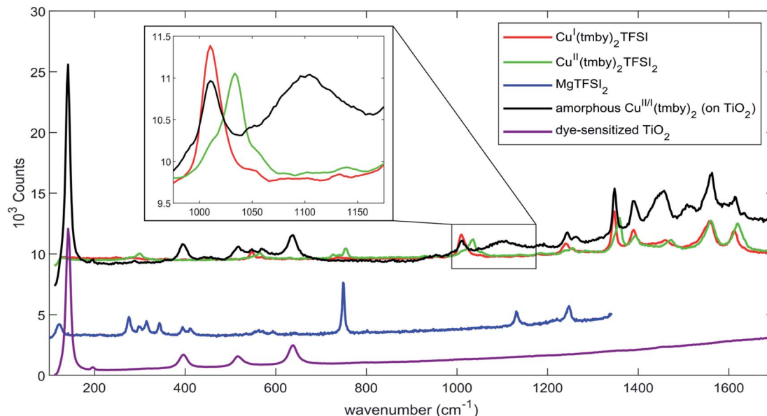
Fig. 4 Raman spectra of \text{Cu}^{\text{I/I}}(\text{tmbly})_2 \text{TFSI}_{(2)} and \text{MgTFSI}_2 (powders), DSCs sensitized with the XY1:L1 sensitizer combination as well as (sensitized) DSCs containing amorphous \text{Cu}^{\text{I/I}}(\text{tmbly})_2 \text{TFSI}_{(2)} hole transport material. The two latter spectra were recorded inside the 'sandwich' DSC. Spectra are offset for clarity.
