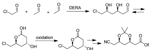
Scheme 19 Enzymatic C–C bond forming reactions.
