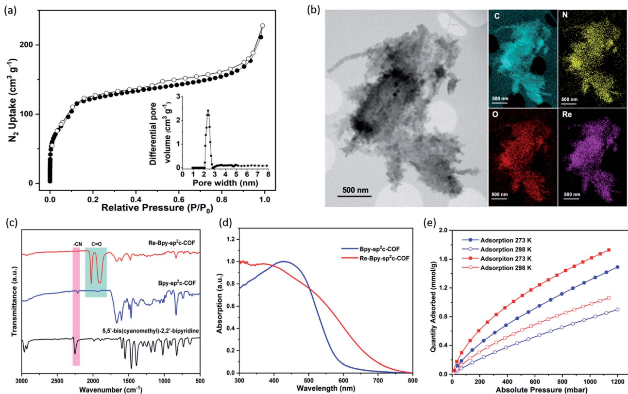
Fig. 2 (a) N_2 Adsorption (filled dots) and desorption (open dots) isotherm profiles of Bpy\text{-}sp^2c\text{-COF} measured at 77 K. Inset: profile of the calculated pore size distribution of Bpy\text{-}sp^2c\text{-COF} ; (b) STEM images and EDX mapping of Re\text{-}Bpy\text{-}sp^2c\text{-COF} ; (c) FT-IR Spectra of Bpy\text{-}sp^2c\text{-COF} , Re\text{-}Bpy\text{-}sp^2c\text{-COF} and 5,5'-bis(cyanomethyl)-2,2'-bipyridine; (d) Solid-state reflectance UV-vis spectra; (e) CO_2 adsorption isotherms of Bpy\text{-}sp^2c\text{-COF} (blue) and Re\text{-}Bpy\text{-}sp^2c\text{-COF} (red).
