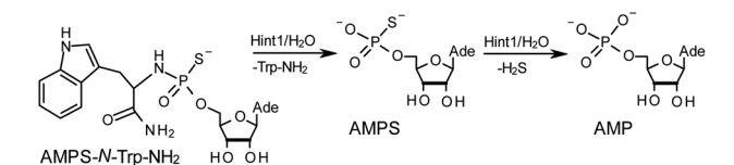
Scheme 3 The HINT1 catalyzed hydrolysis of adenosine-5'- O -(( L -tryptophan amide- N\alpha -yl)-phosphoramidothioate) (AMPS-Trp-NH 2 ), followed by desulfuration of the AMPS intermediate leading to the formation of adenosine-5'- O -phosphate.
