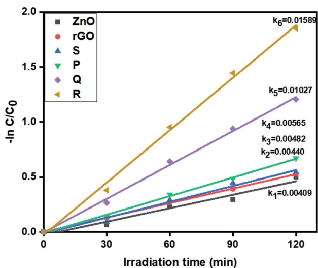
Fig. 7 The kinetic data of ZnO, rGO and ZnO/rGO composites for Cr(vi) reduction (120 min of irradiation time, 50 mg L -1 of catalyst, 20 ppm of Cr(vi)).
