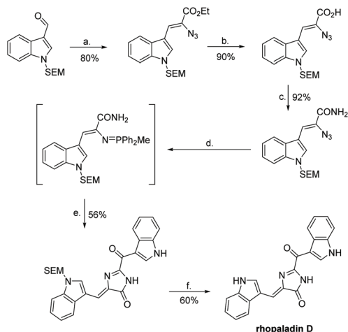
Scheme 34 First total synthesis of rhopaladin D. Reagents (a) \text{N}_3\text{CH}_2\text{COOEt} , NaEtO, EtOH, -15^\circ\text{C} ; (b) LiOH, THF, \text{H}_2\text{O} ; (c) carbonyldiimidazole (CDI), \text{NH}_3 , DMF; (d) \text{PPh}_2\text{Me} , THF; (e) indolyl-3-glyoxytyl chloride, polymer-bound BEMP, THF; (f) TBAF, THF, reflux.
