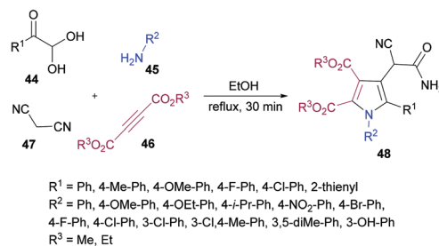
Scheme 10 Four-component domino synthesis of polysubstituted pyrroles.
