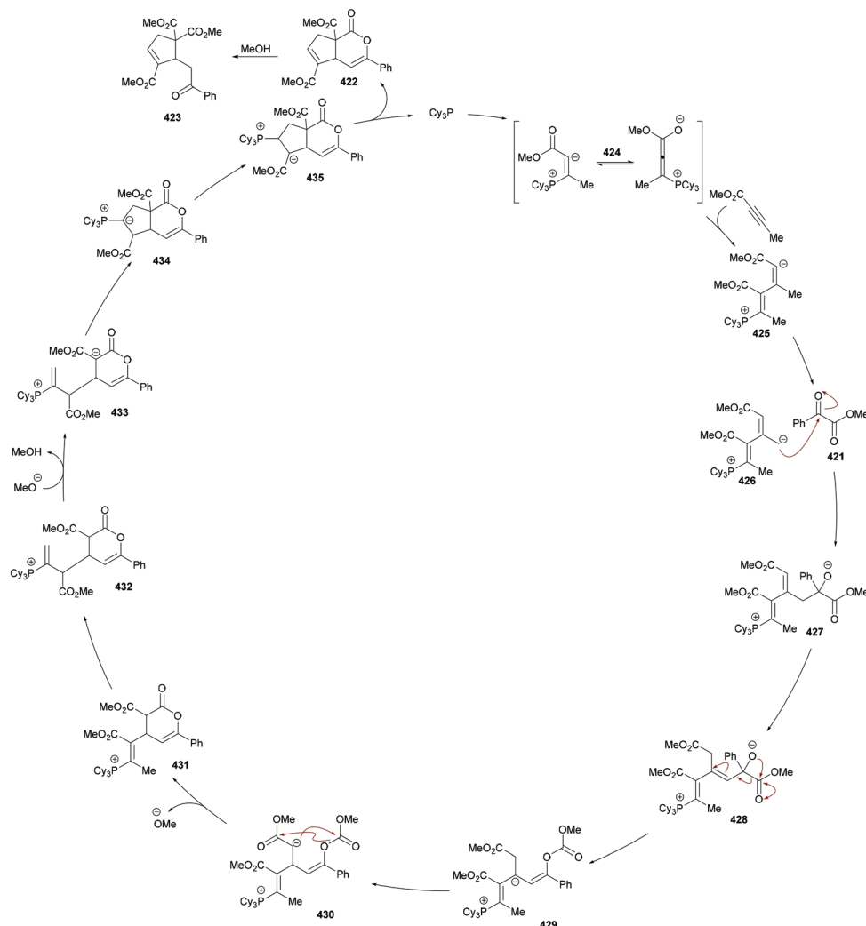
Scheme 106 Proposed mechanism for the formation of cyclopentene fused dihydropyrrone 422 and monocyclic five-membered product 423 .
