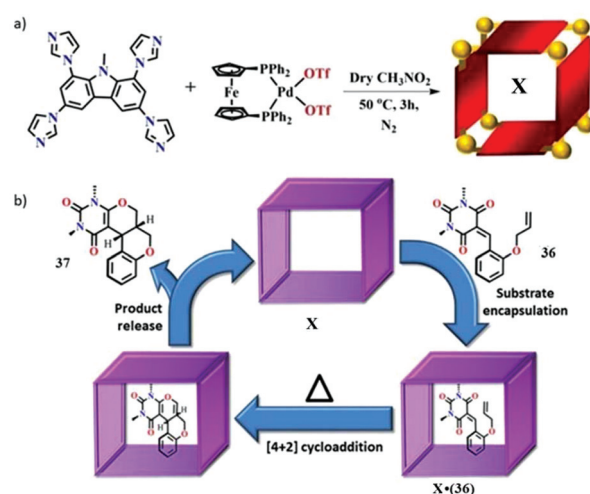
Fig. 51 (a) Synthesis of the 'symmetrized' molecular tube-shaped cage X. (b) Plausible mechanism of intramolecular hetero Diels-Alder reaction within cage X. Reproduced with permission from ref. 152. Copyright 2017, John Wiley & Sons, Ltd.
