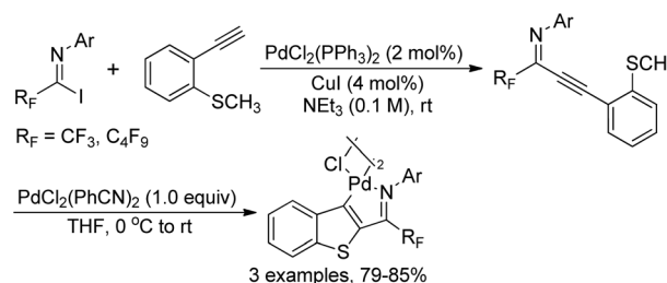
Scheme 38 Synthesis of benzothienophene-based palladacycles.
