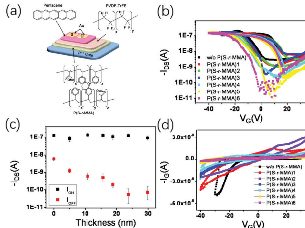
Fig. 11 (a) Schematic illustration of a bottom gate FeFET with pentacene as the active layer and bilayered PVDF-TrFE/P(S- r -MMA) as the gate dielectric. (b) Transfer curves ( I_D - V_G ) at V_D = 5 V of pentacene FeFETs with six different P(S- r -MMA) interlayers. The transfer curve of the pentacene FeFET without a P(S- r -MMA) layer is also plotted for comparison. (c) Plots of I_{\text{on/off}} as a function of the P(S- r -MMA) interlayer thickness. While I_{\text{on}} remains similar, I_{\text{off}} gradually decreases with the interlayer film thickness up to approximately 25 nm. (d) I_G - V_G characteristics of the FeFETs simultaneously obtained with the transfer characteristics showing that the gate leakage current becomes significantly reduced with the thickness of the interlayer. Reproduced with permission. 65 Copyright 2009, Elsevier.
