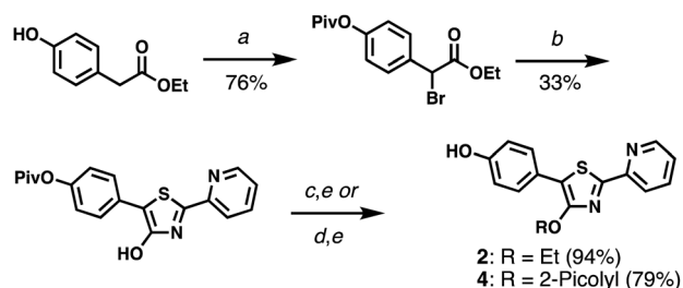
Scheme 1 Synthesis of HPPT derivatives 2 and 4. (a) (i) \text{PivCl} , DMAP, pyridine; (ii) NBS, AIBN, TBT, 80^\circ\text{C} . (b) 2-Pyridylthioamide, EtOH, 90^\circ\text{C} ( \mu\text{W} ). (c) EtI, \text{K}_2\text{CO}_3 , acetone. (d) 2-PicBr-HBr, \text{K}_2\text{CO}_3 , acetone. (e) \text{K}_2\text{CO}_3 , MeOH. See ESI† for reagent abbreviations.
